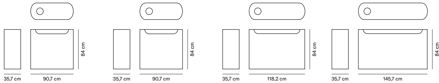
MEV-02-TC Capacity: 226 L (2 x 113 L) NET: 32 kg | GROSS: 33 kg
